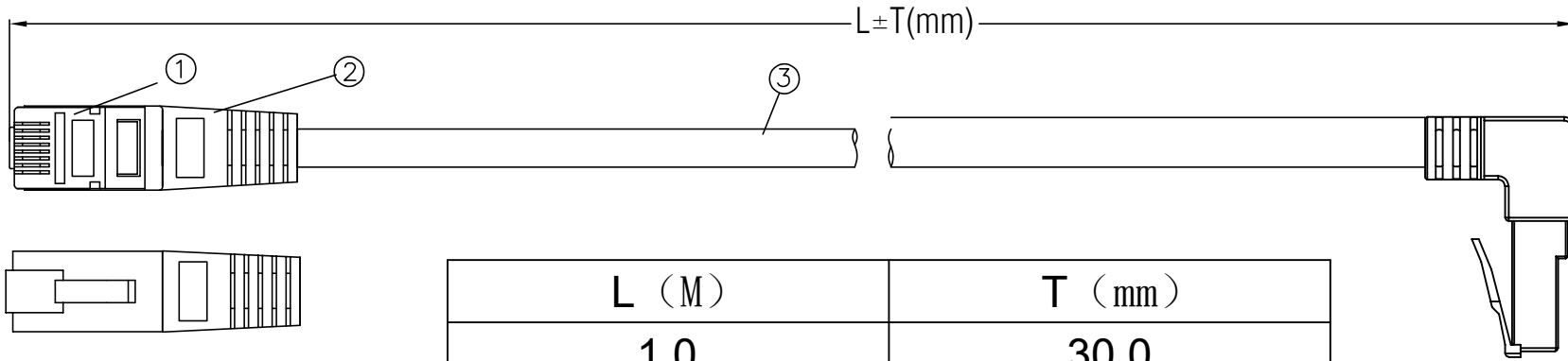
A FRONT VIEW
